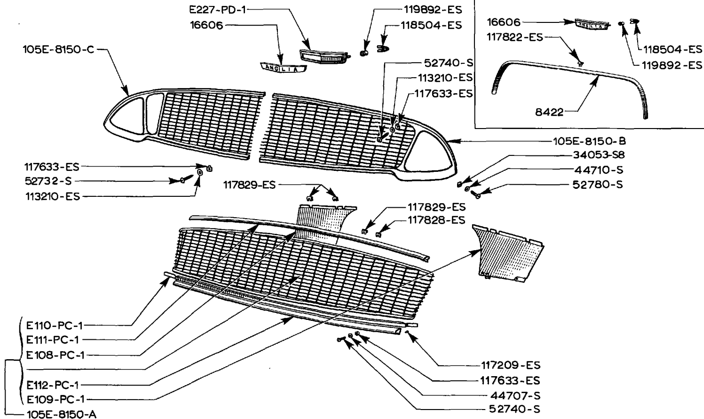
RADIATOR GRILLE-SALOON AND ESTATE CAR
