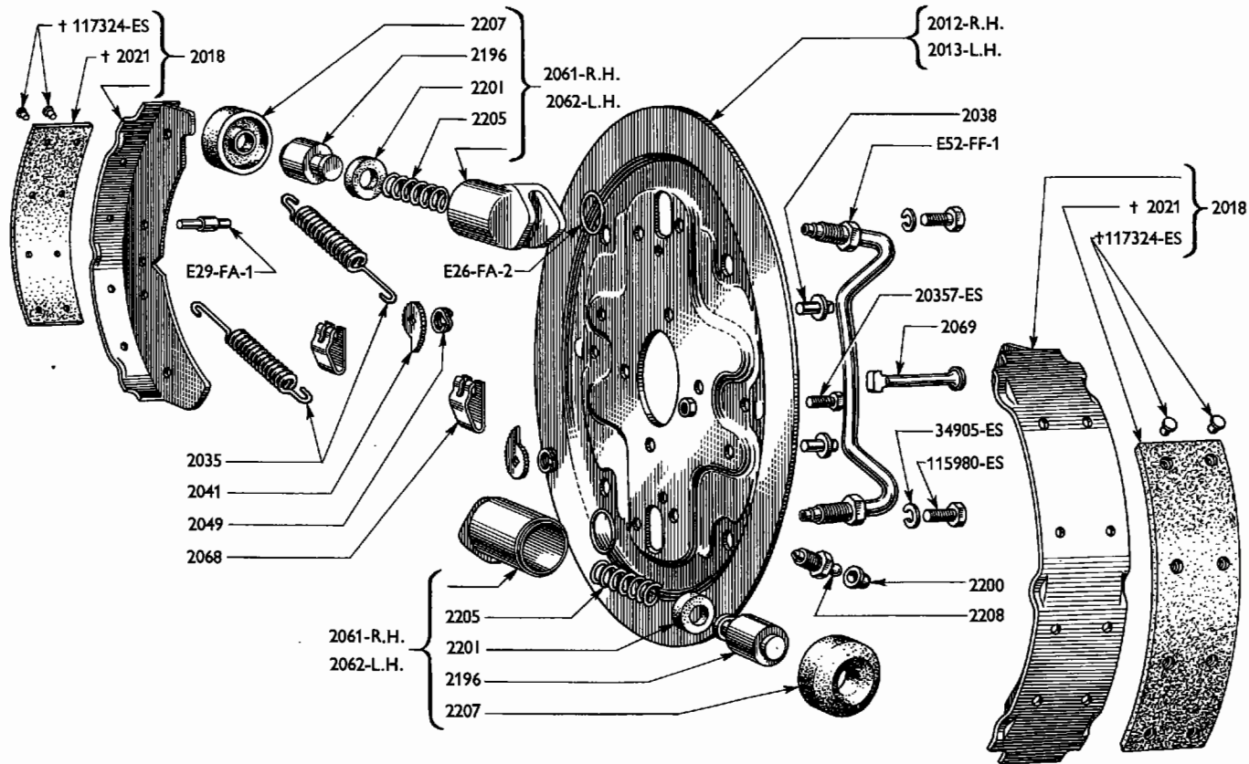
FRONT BRAKE PLATE—1198 c.c. MODEL
