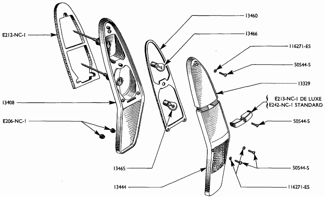
REAR LAMP — ESTATE CAR
