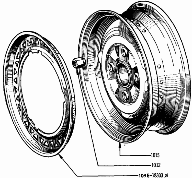
WHEEL AND HUB CAP
