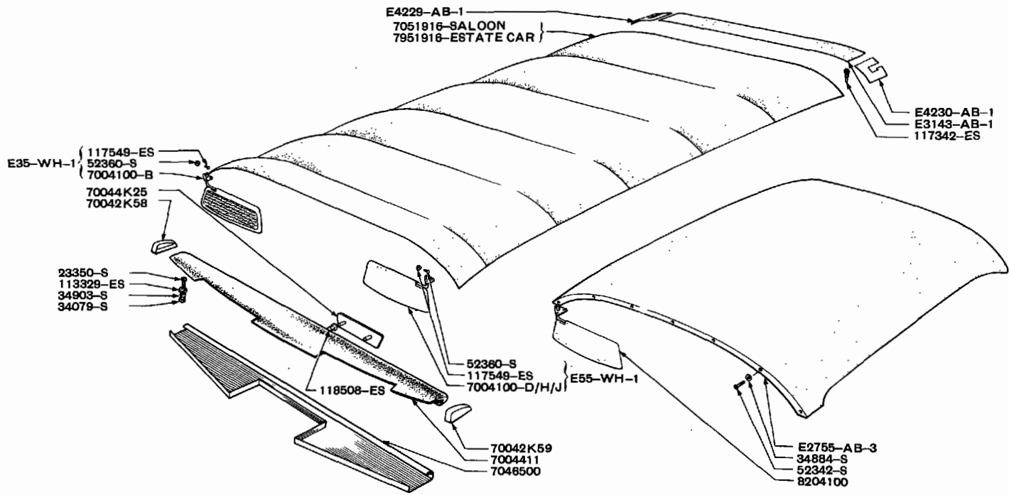
FRONT END AND ROOF TRIM
