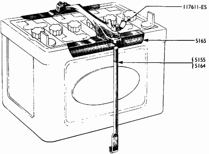
BATTERY CLAMP
