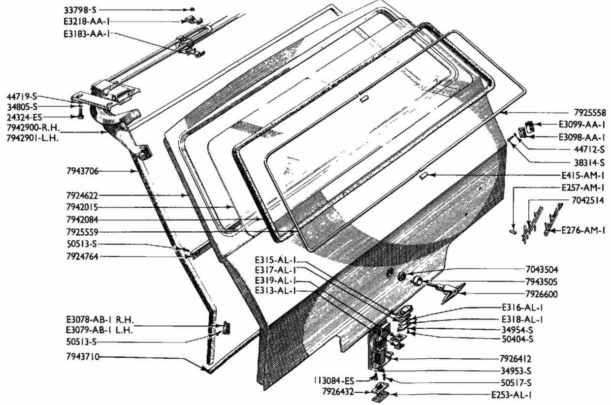
REAR DOOR-ESTATE CAR
