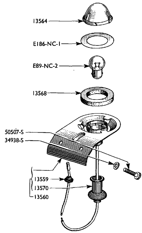
LICENCE PLATE ILLUMINATION LAMP
