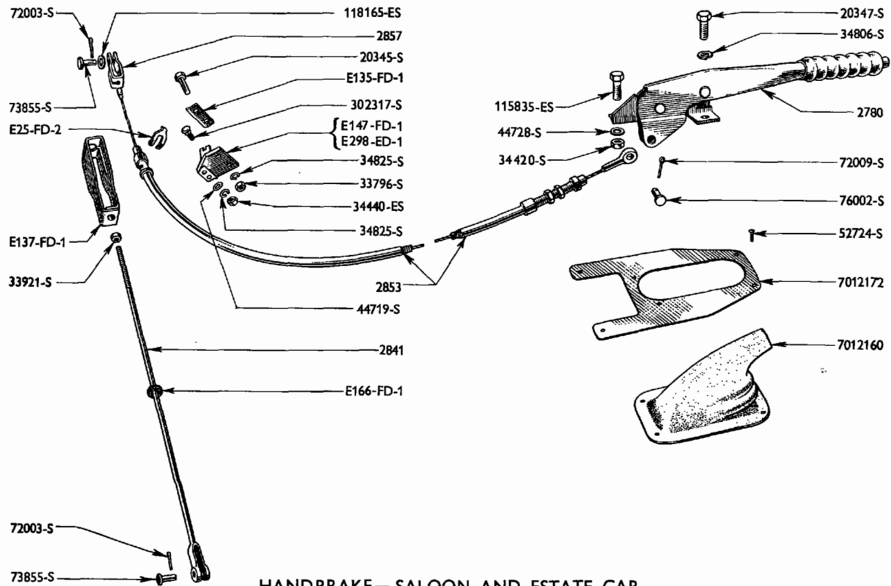
HANDBRAKE—SALOON AND ESTATE CAR
