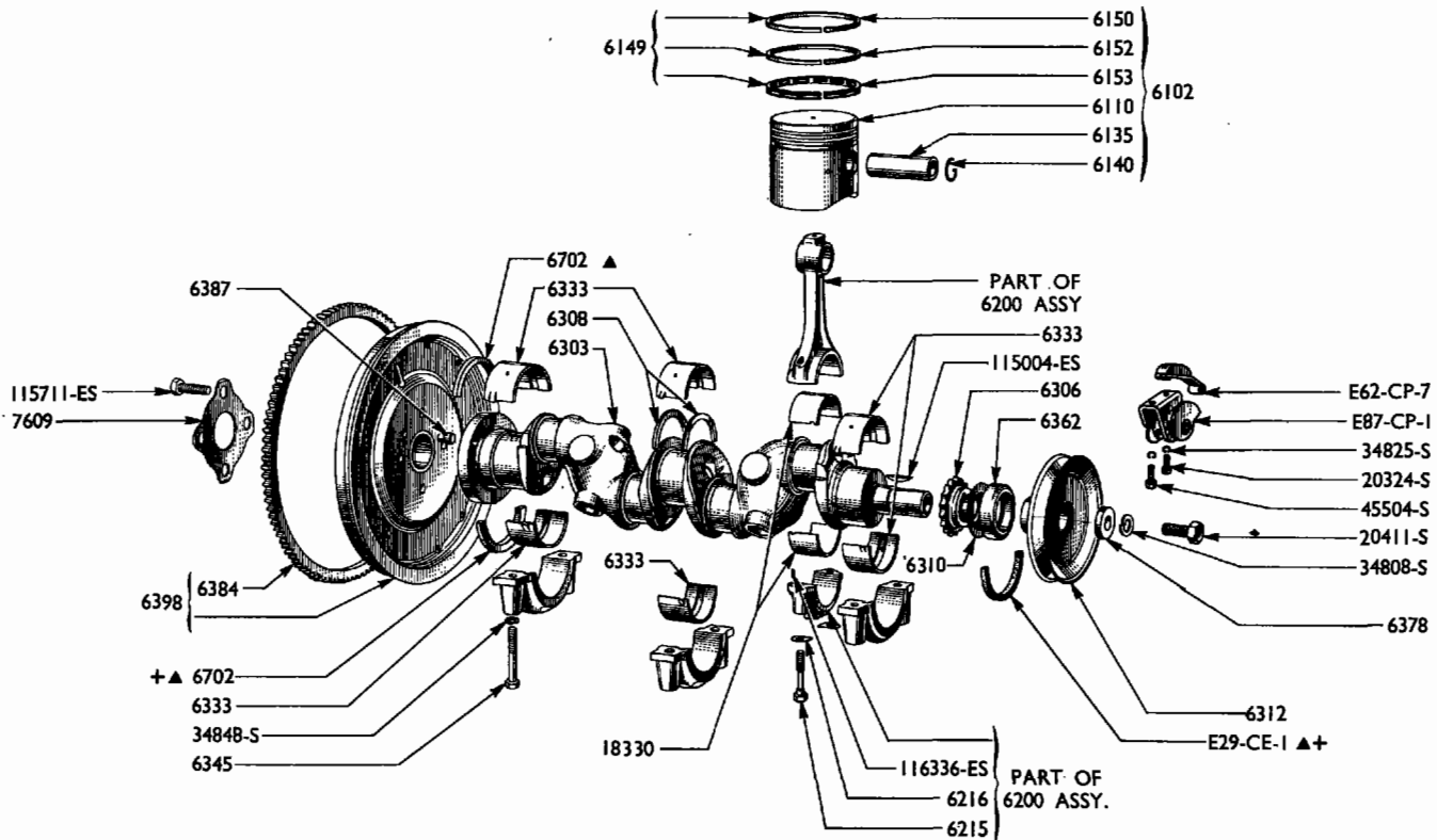
ENGINE INTERIOR
