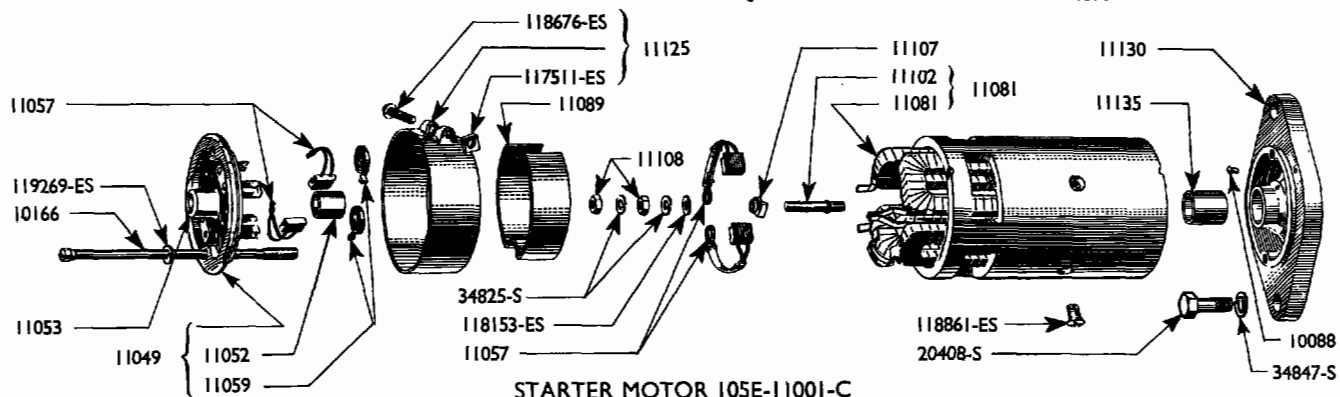
STARTER MOTOR 105E-11001-C
