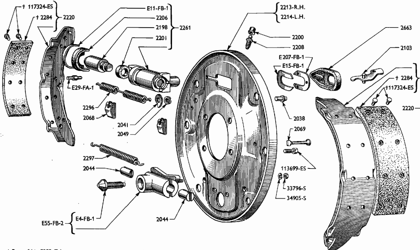
REAR BRAKE PLATE—1198 c.c. MODEL
