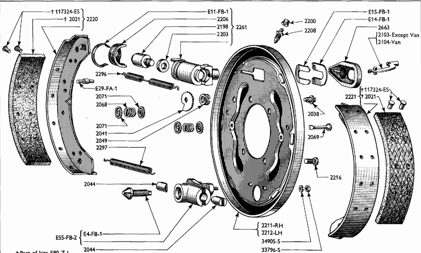
REAR BRAKE PLATE — 997 c.c. MODEL
