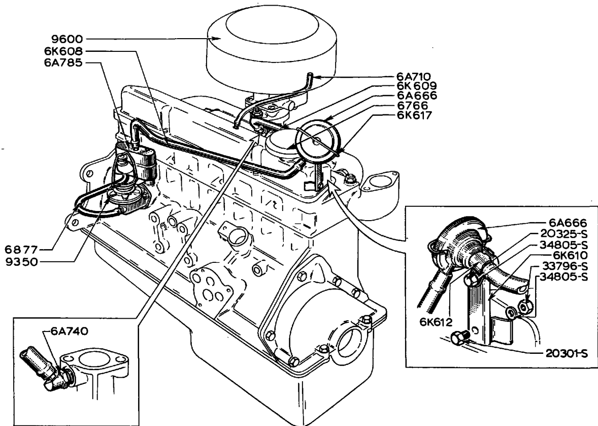
CRANKCASE EMISSION CONTROL SYSTEM
