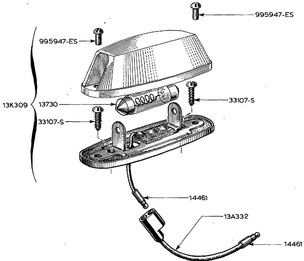
SIDE FLASHER -ITALY
