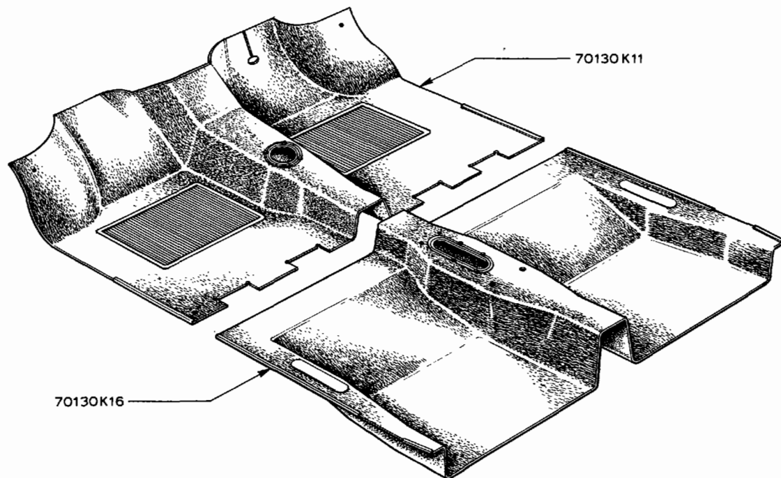
FLOOR TRIM-SALOON
