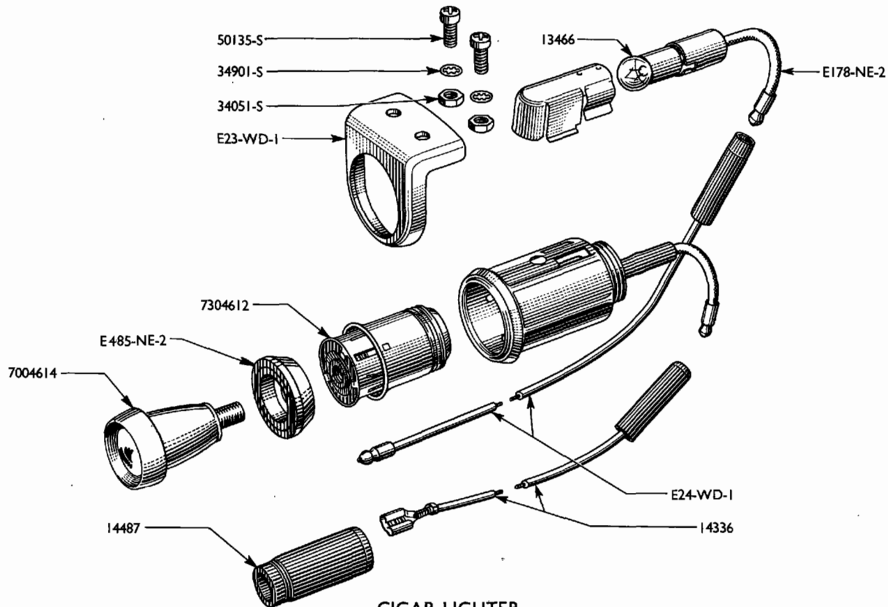
CIGAR LIGHTER
