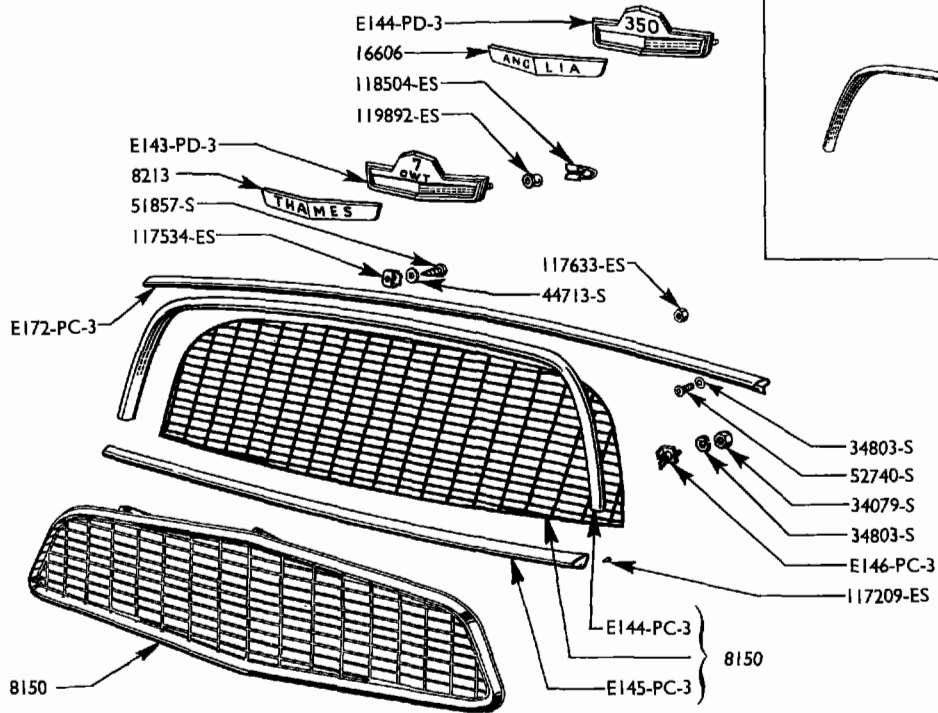
RADIATOR GRILLE - VAN AND U.S.A.
