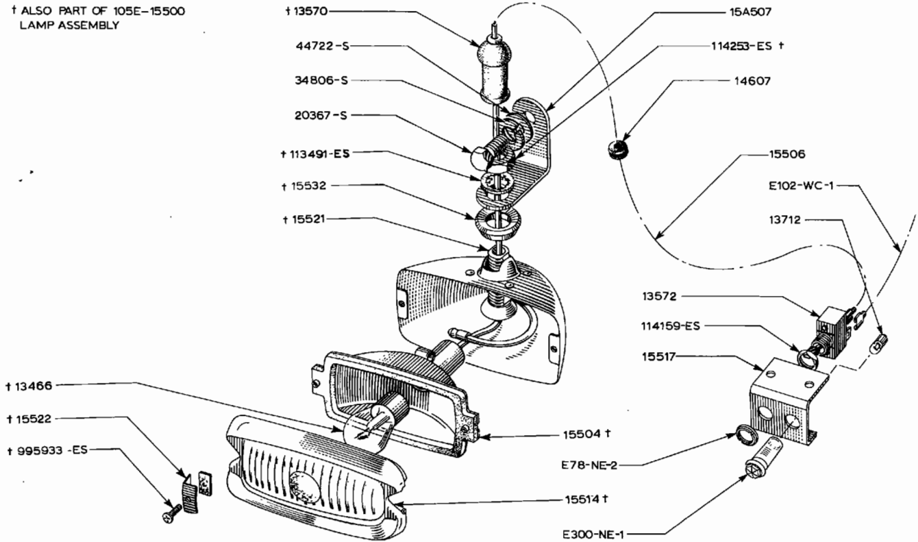
REVERSING LAMP
