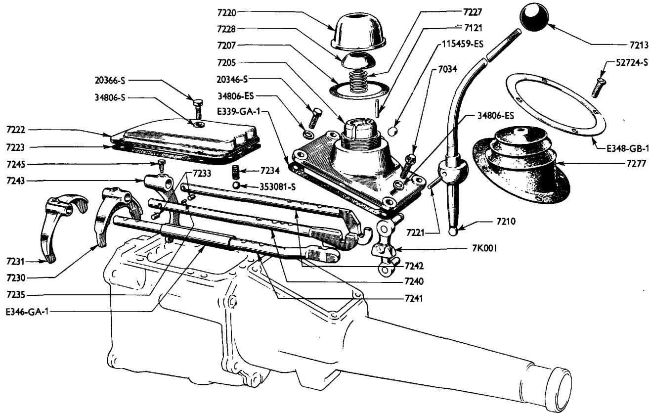
GEARBOX—FLOOR CHANGE—1198 cc.
