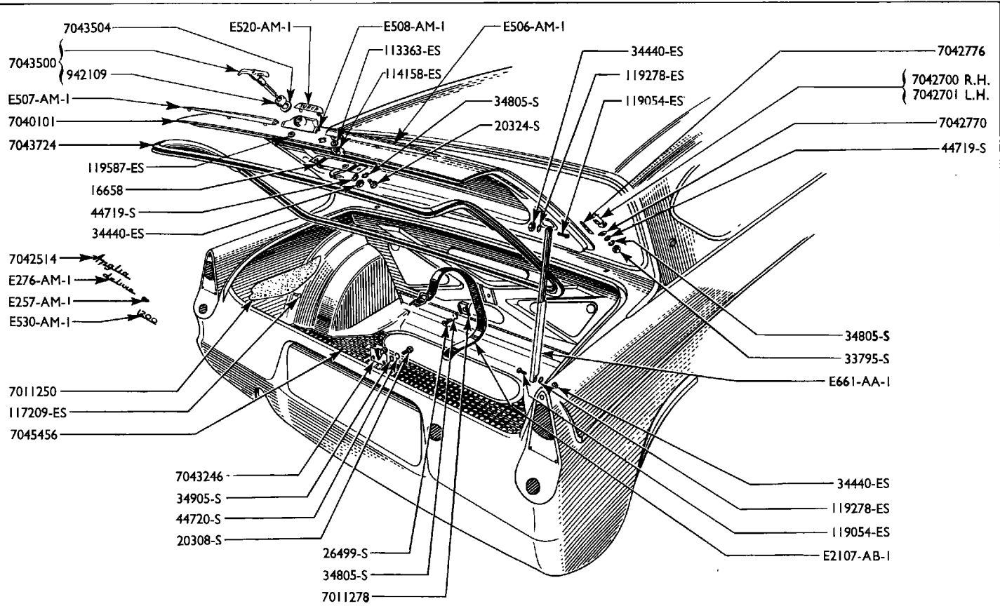
LUGGAGE COMPARTMENT
