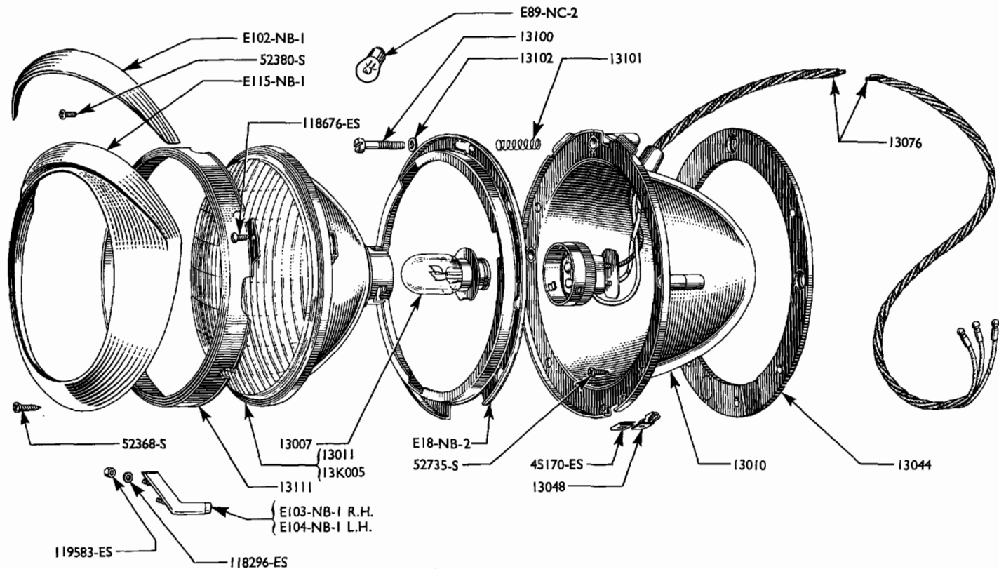
HEADLAMP—SEMI SEALED BEAM—AND BEZELS
