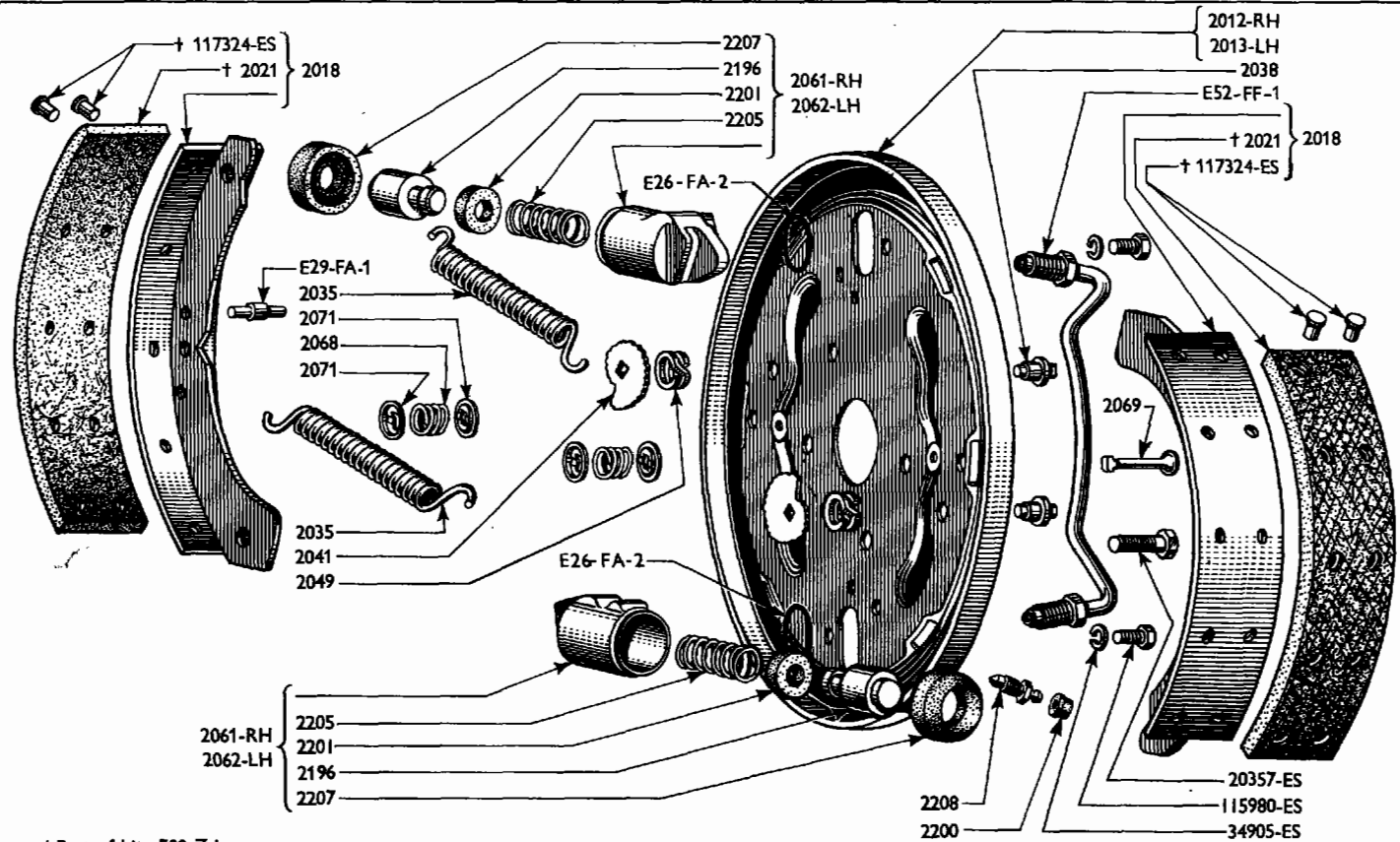
FRONT BRAKE PLATE — 997 c.c. MODEL
