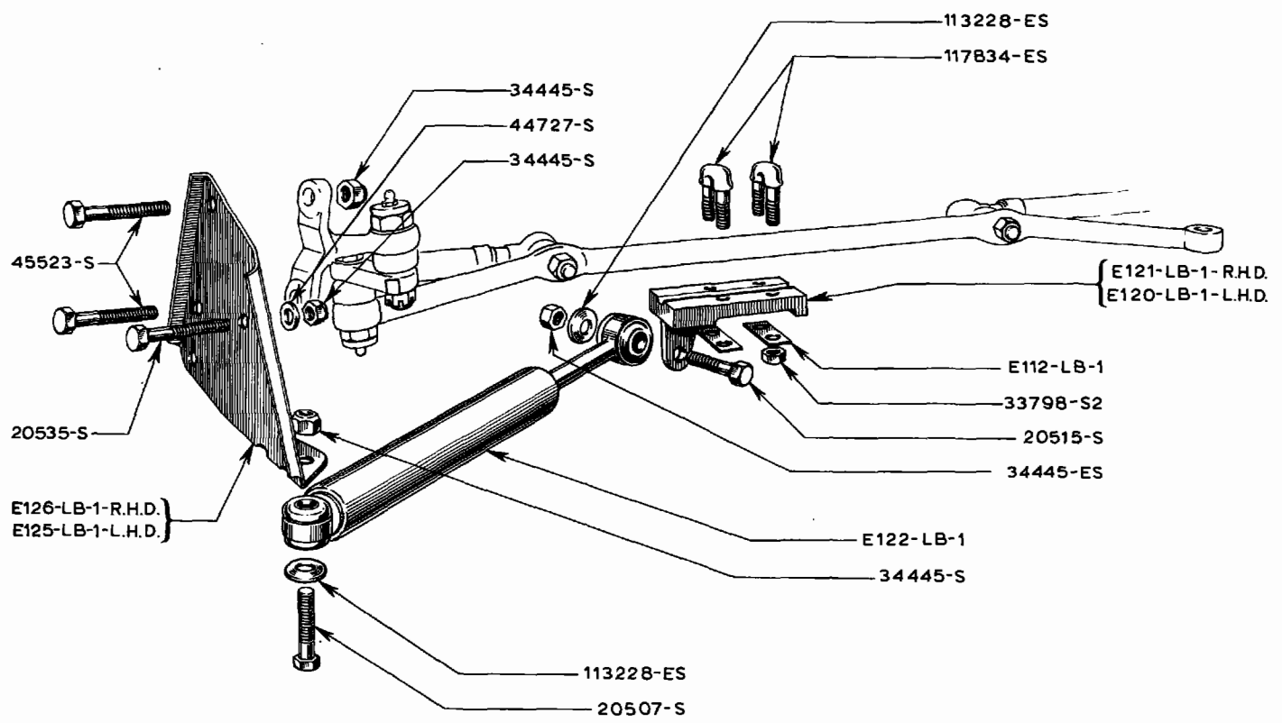
STEERING DAMPER (R.H.D. SHOWN)
