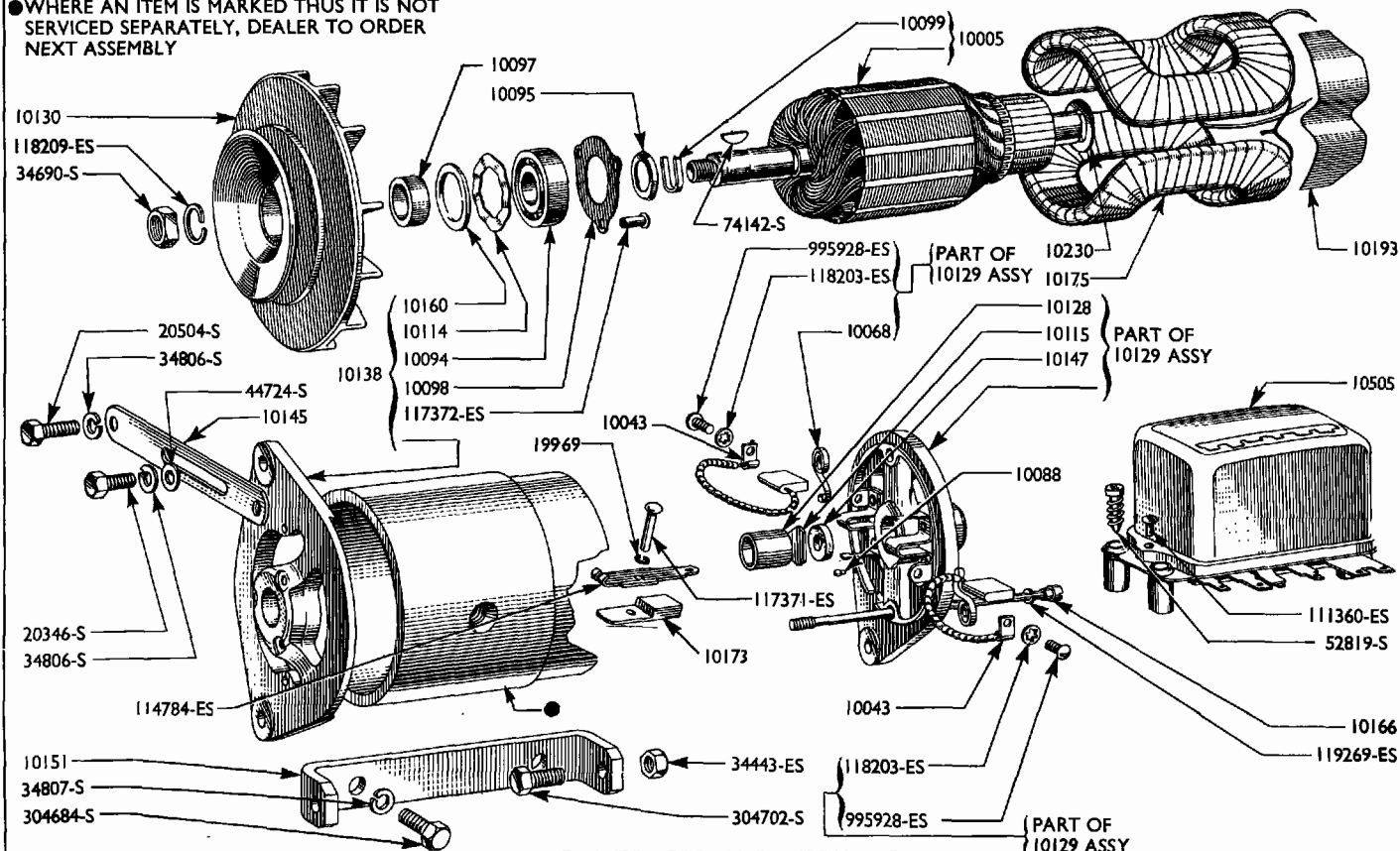
GENERATOR AND REGULATOR
