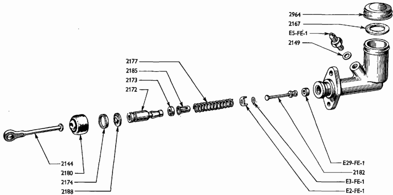
CLUTCH AND BRAKE MASTER CYLINDER
