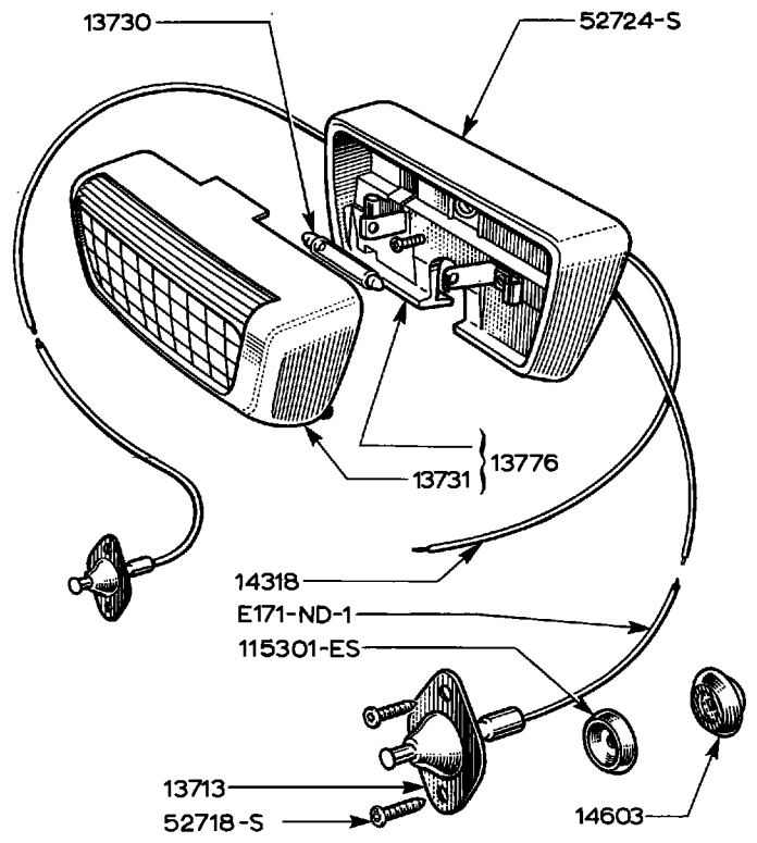
INTERIOR LAMP WIRING AND COURTESY SWITCH
