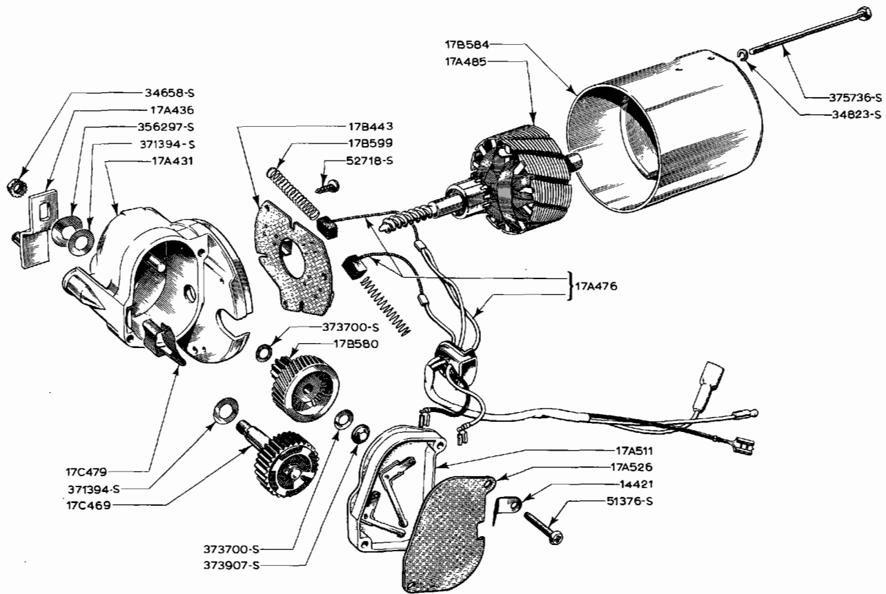
WINDSCREEN WIPER MOTOR-AUTOLITE
