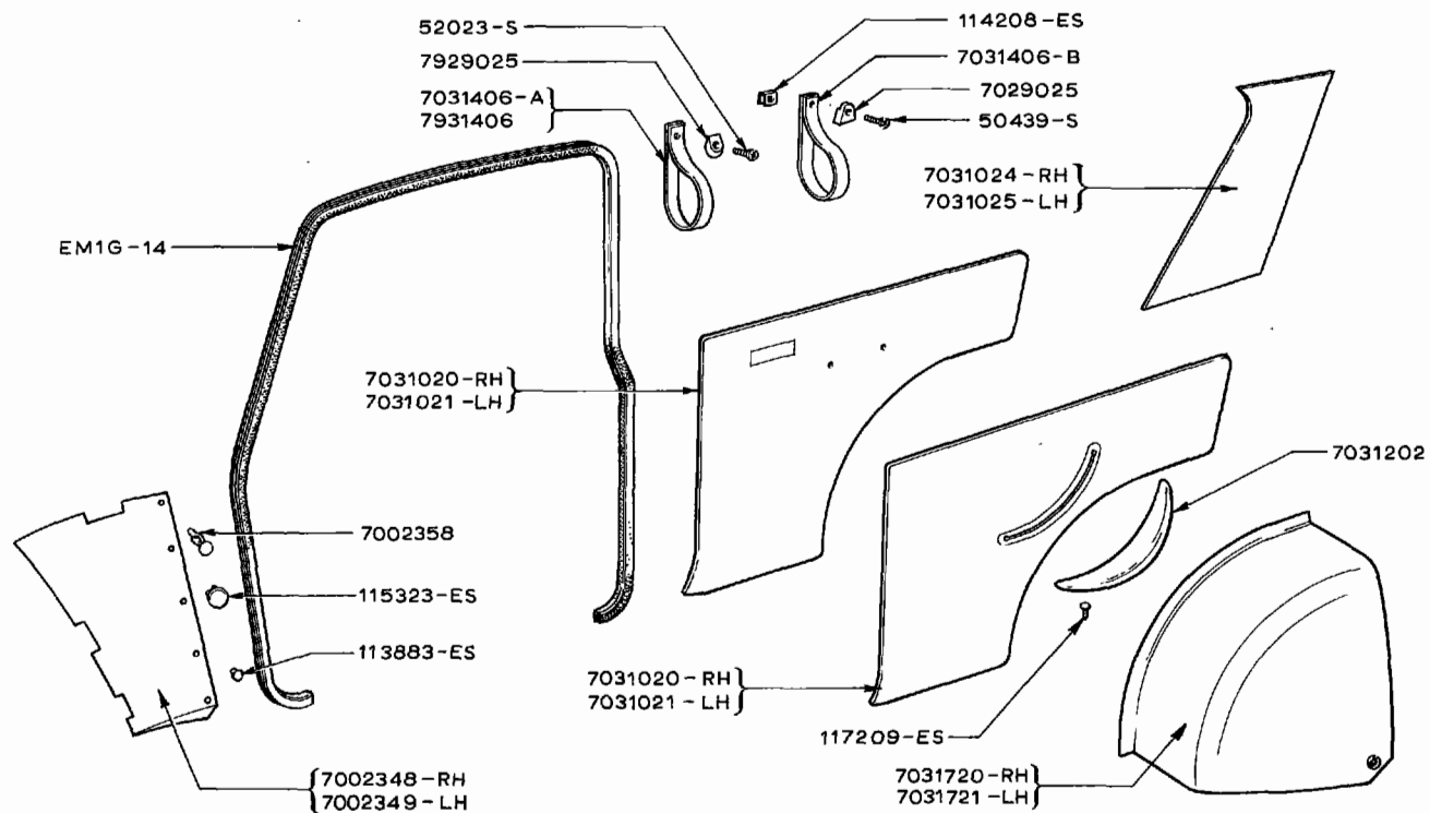
SIDE TRIM SALOON
