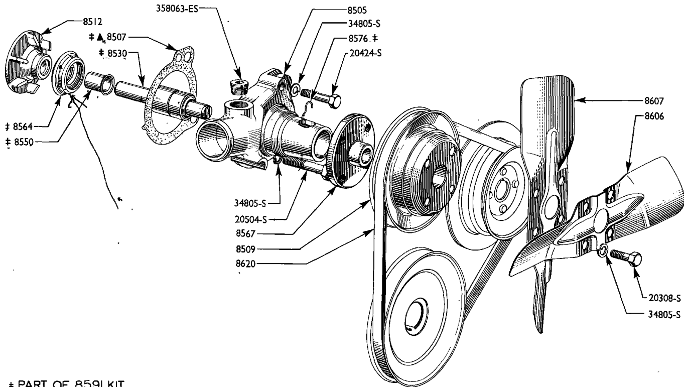
WATER PUMP, FAN AND FAN BELT
