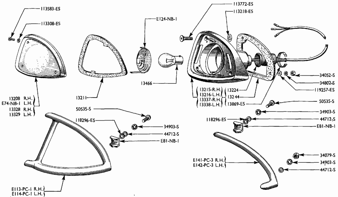
WING LAMP AND FRONT FLASHER-EXCEPT GERMANY AND EIRE -USED 9/59/65/6 FRONT FLASHER-GERMANY FROM 9/59, EIRE FROM 4/64/ AND DOMESTIC FROM 6/65/-
