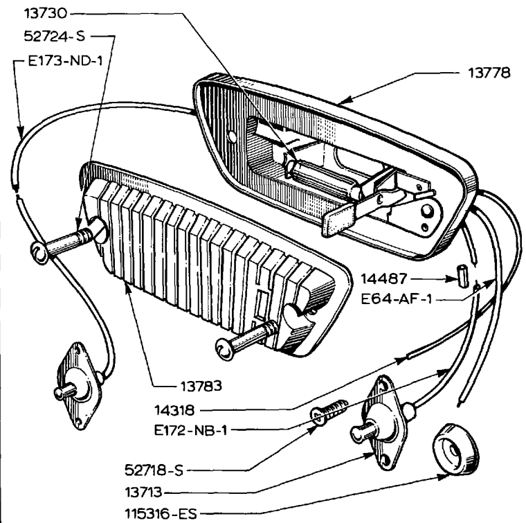
INTERIOR LAMP, WIRING AND COURTESY SWITCH-ESTATE CAR 8/63/
