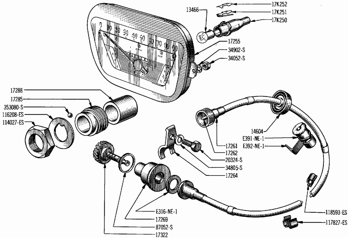
SPEEDOMETER
