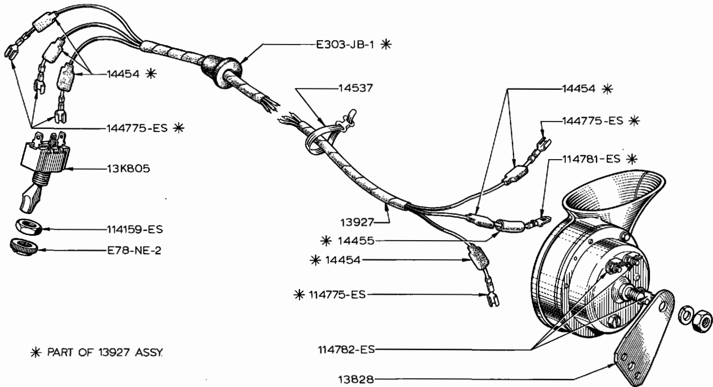
DUAL TONE HORN - FRANCE ONLY
