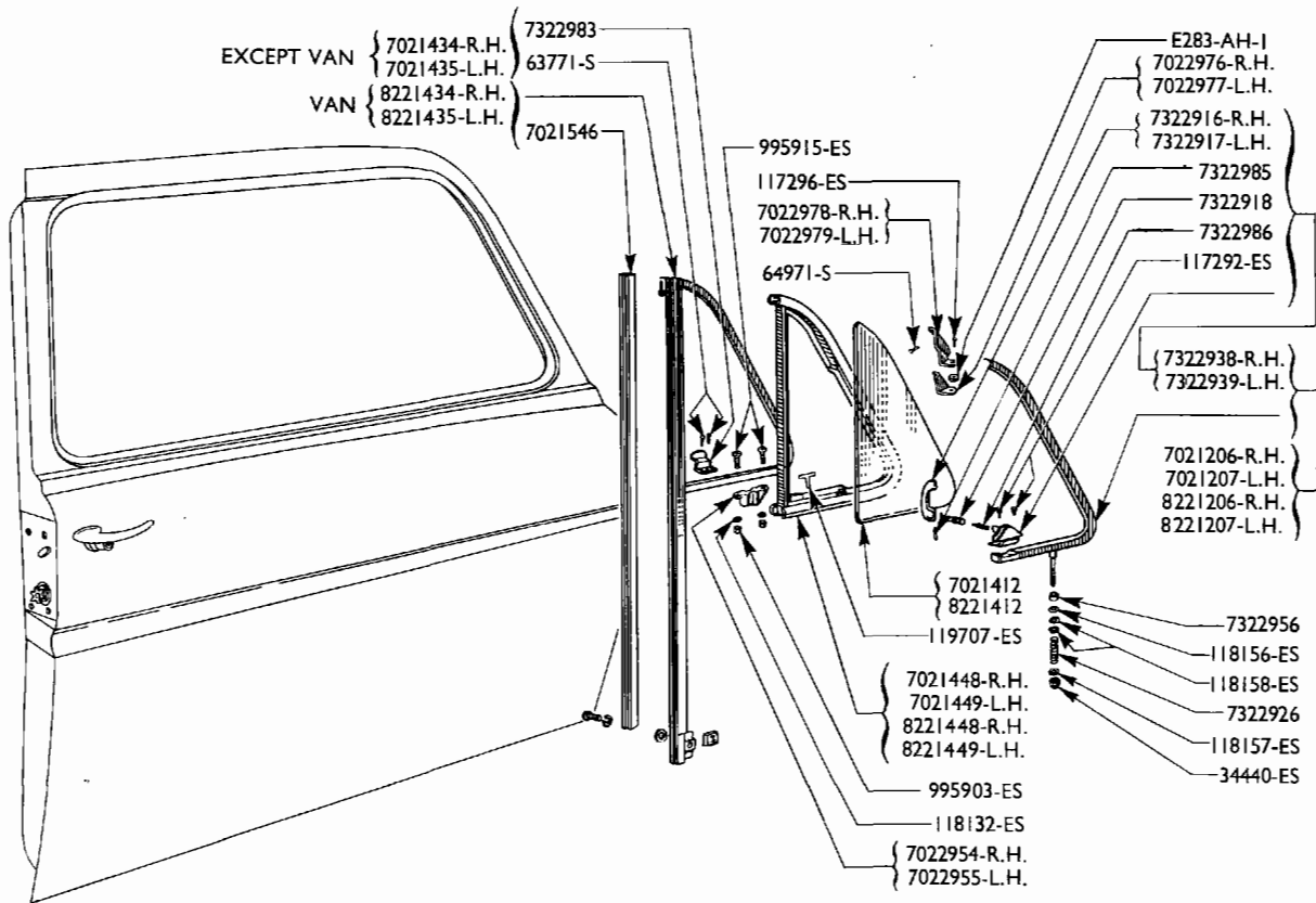
FRONT DOOR VENT WINDOW
