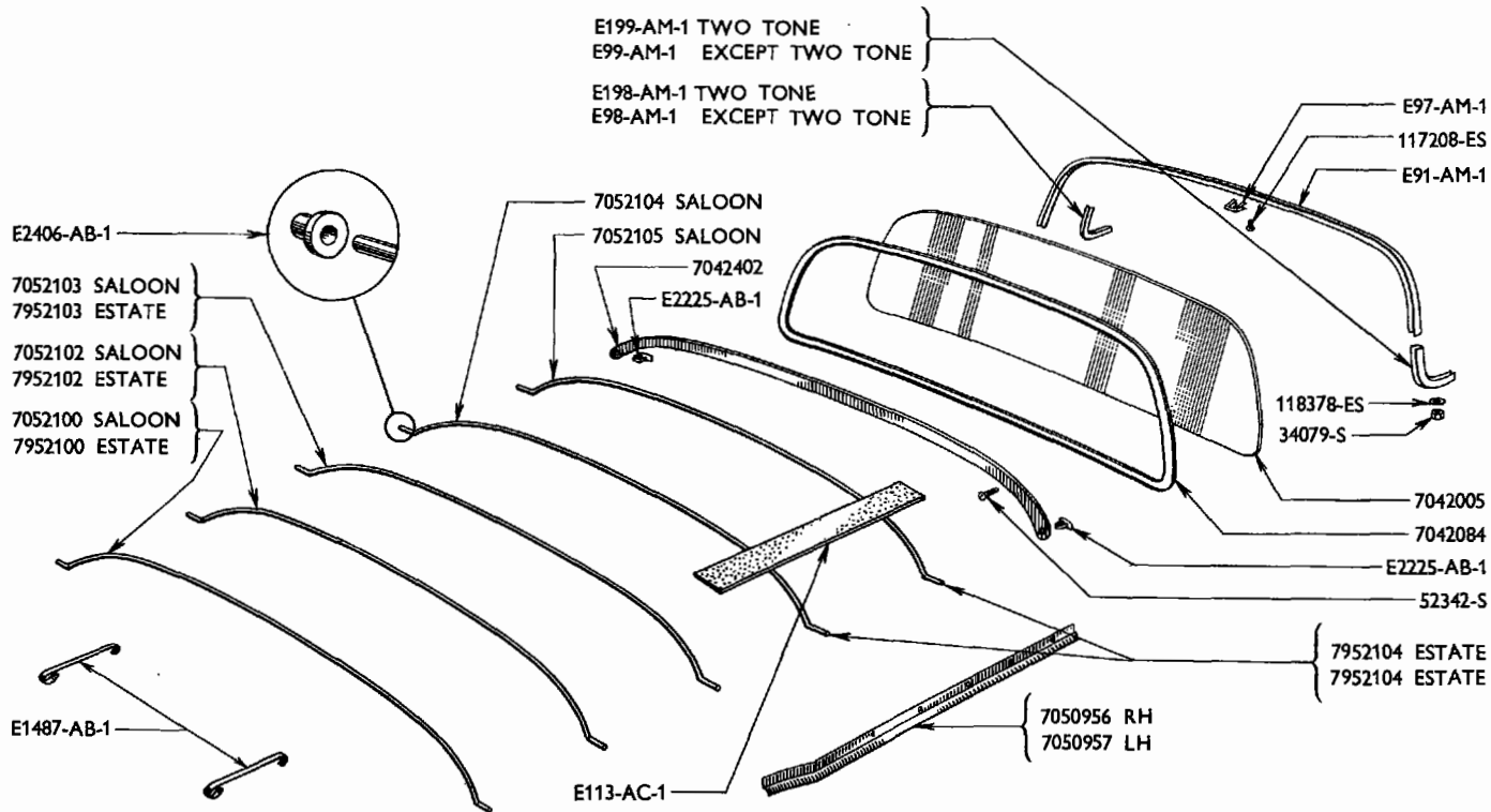
ROOF AND REAR WINDOW—SALOON AND ESTATE CAR
