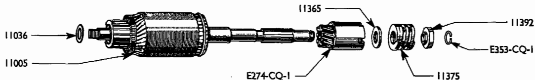
PINION ASSY. USED WITH 105E 11001-B
