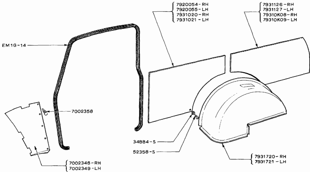
SIDE TRIM ESTATE CAR
