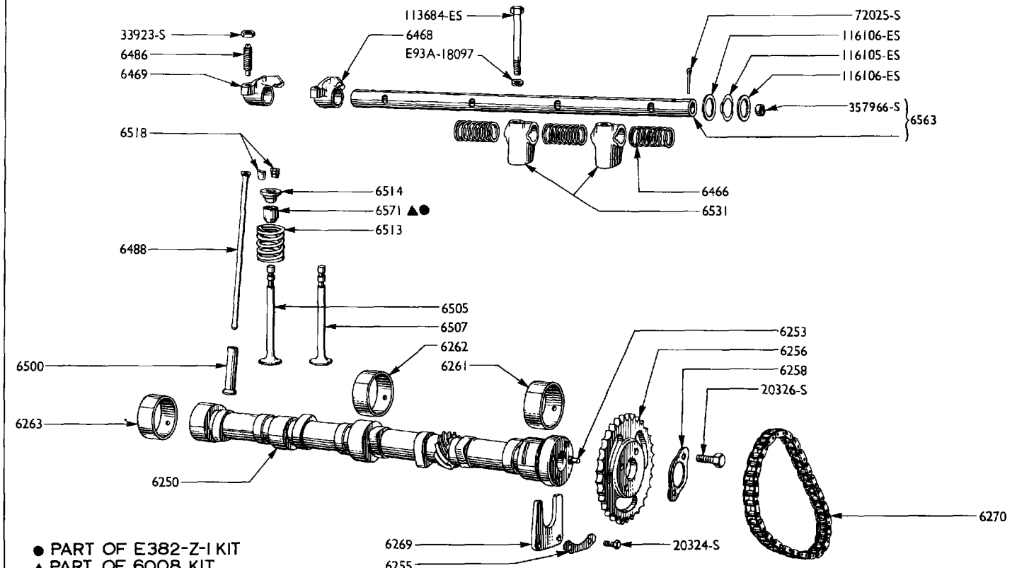
VALVE OPERATING MECHANISM
