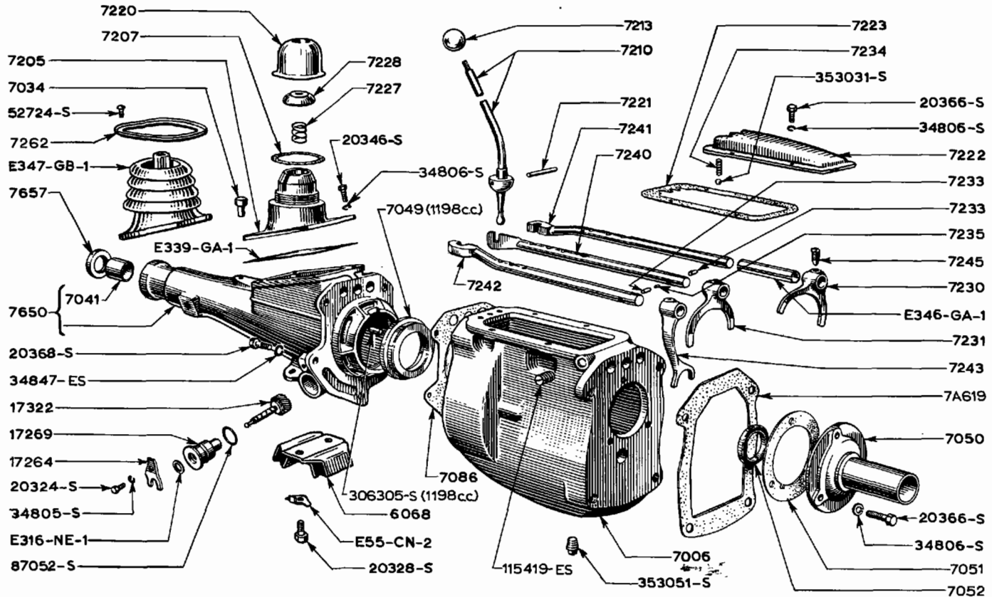
GEARBOX EXTERIOR-FLOOR CHANGE -997 c.c.
