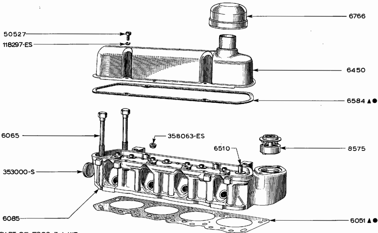
CYLINDER HEAD
