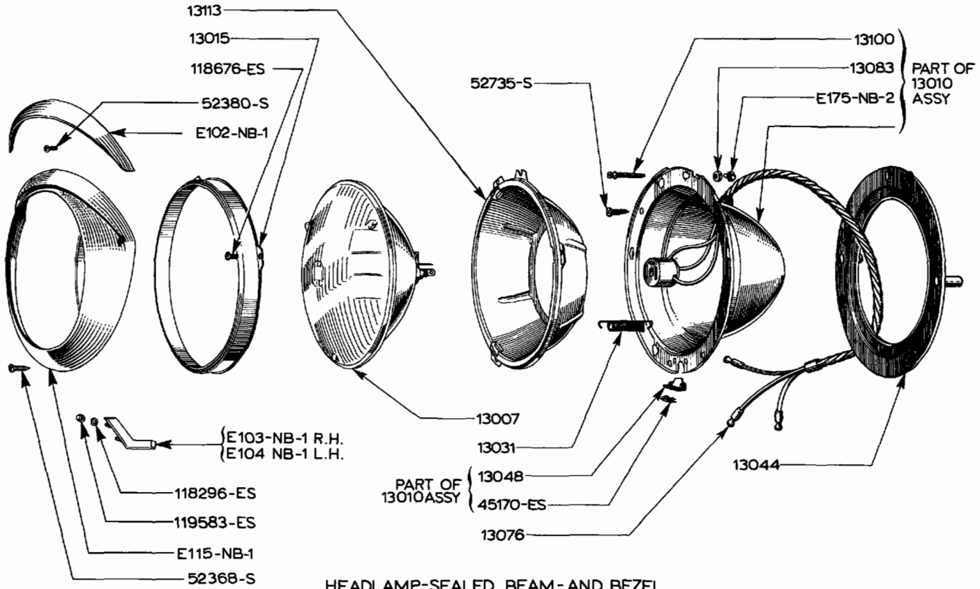
HEADLAMP-SEALED BEAM-AND BEZEL
