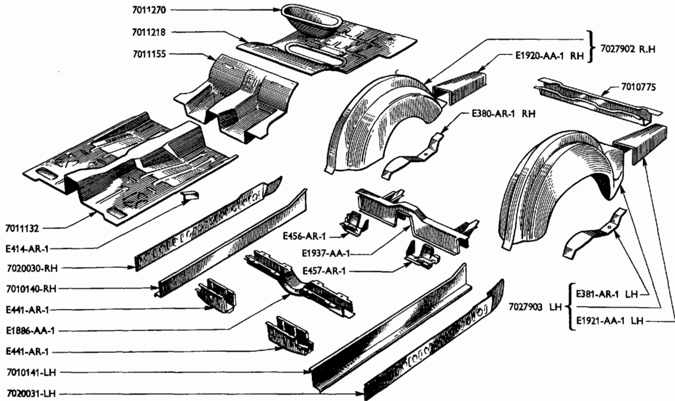
SALOON FLOOR AND MEMBERS
