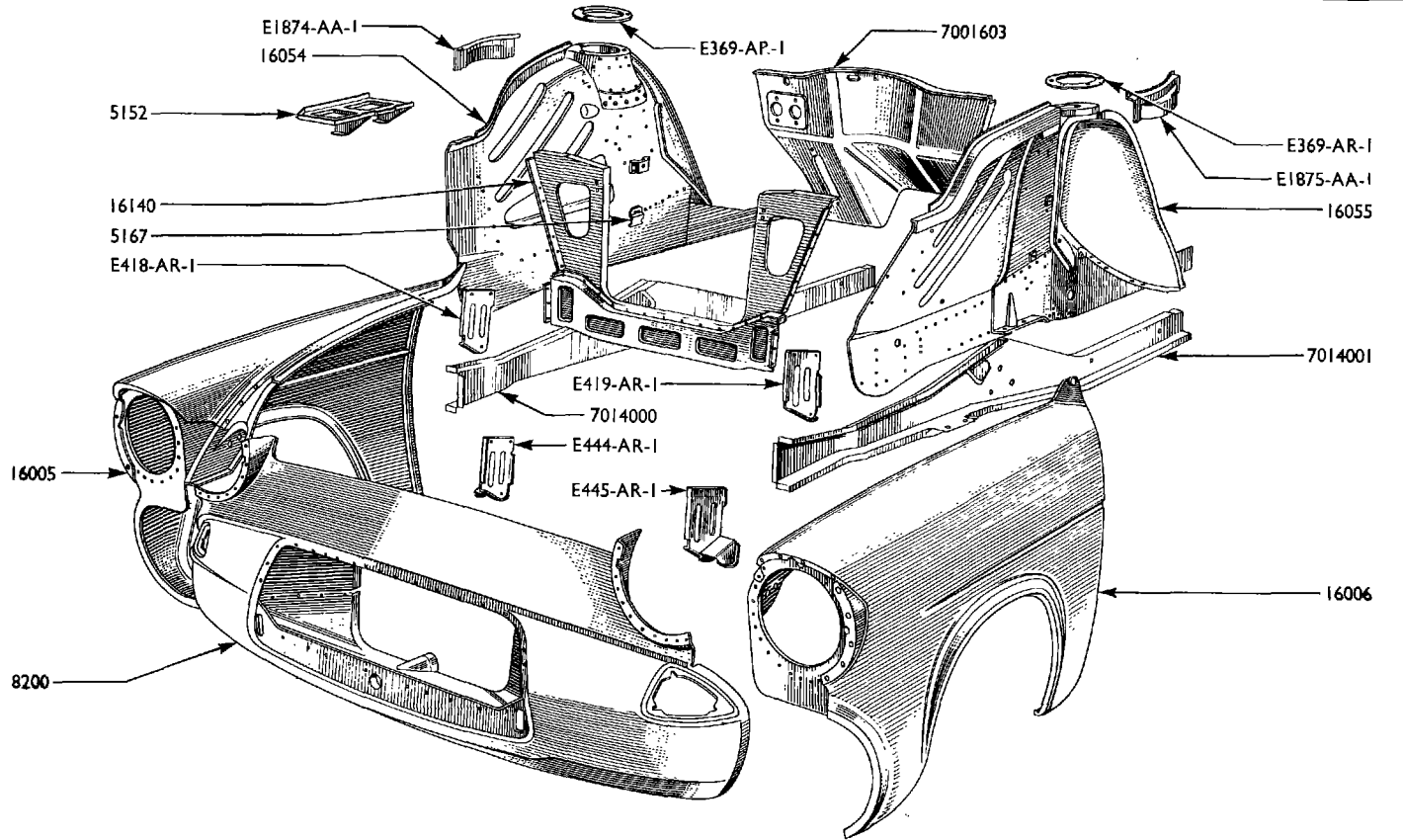
ENGINE COMPARTMENT
