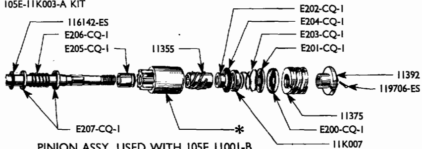
PINION ASSY. USED WITH 105E 11001-B
