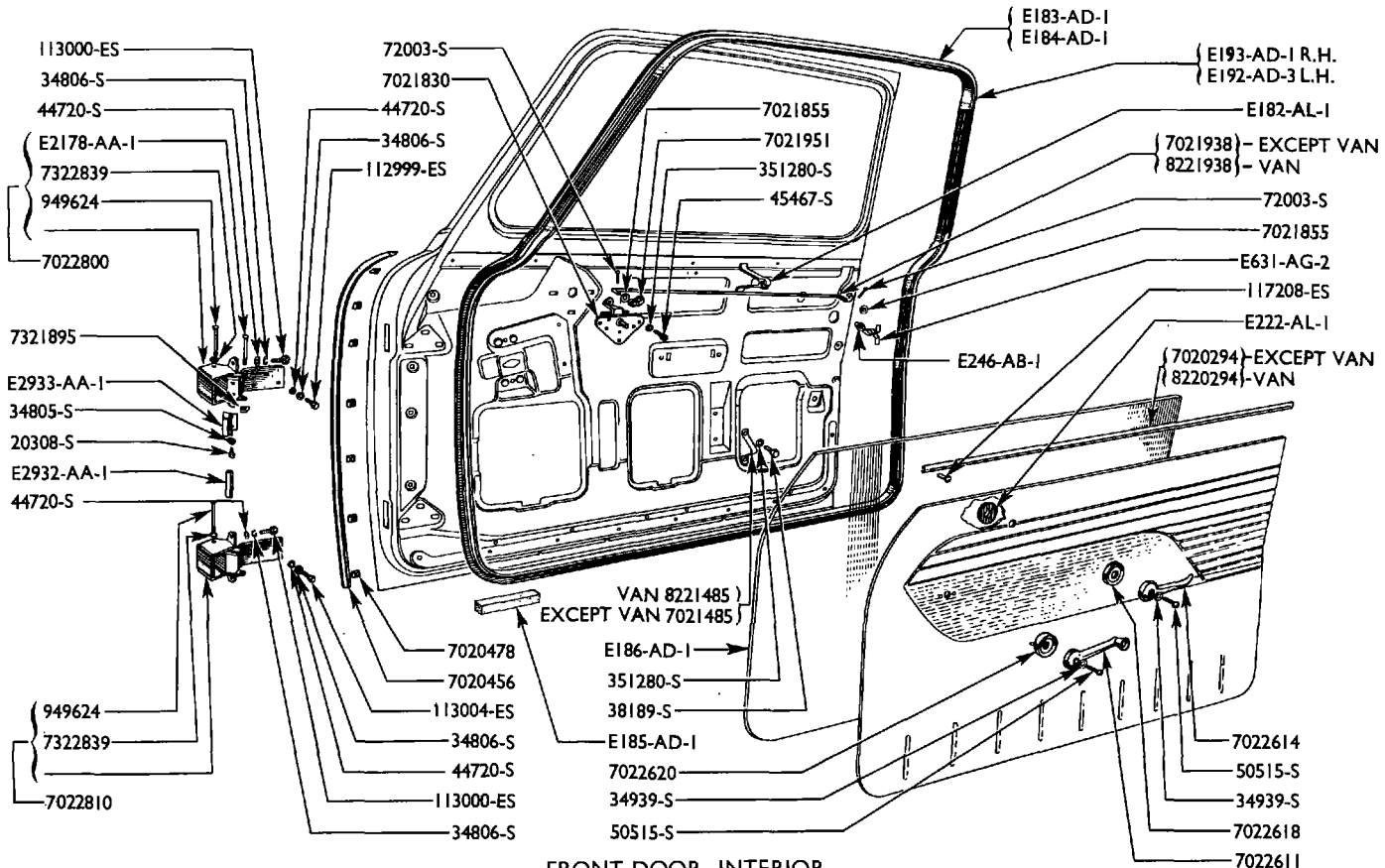
FRONT DOOR - INTERIOR
