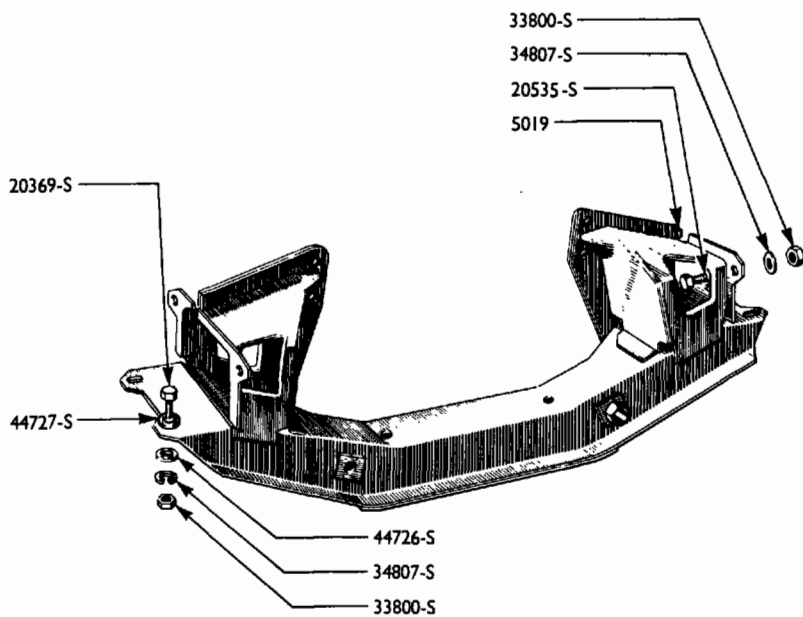
FRONT SUSPENSION CROSSMEMBER
