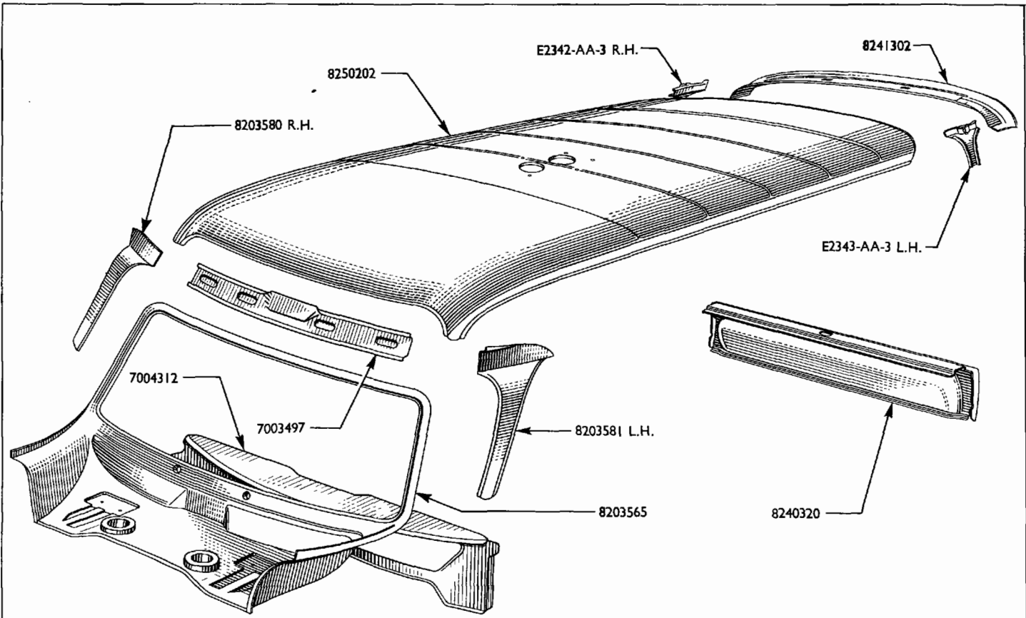
ROOF AND BACK PANEL - VAN
