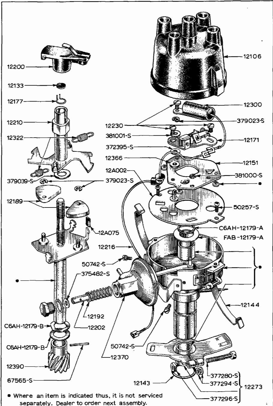
AUTOLITE DISTRIBUTOR
