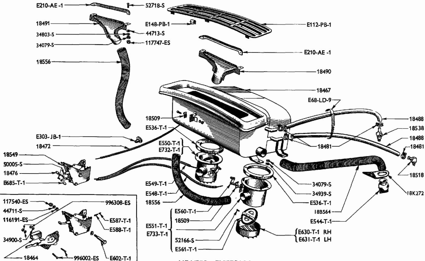
HEATER EXTERIOR
